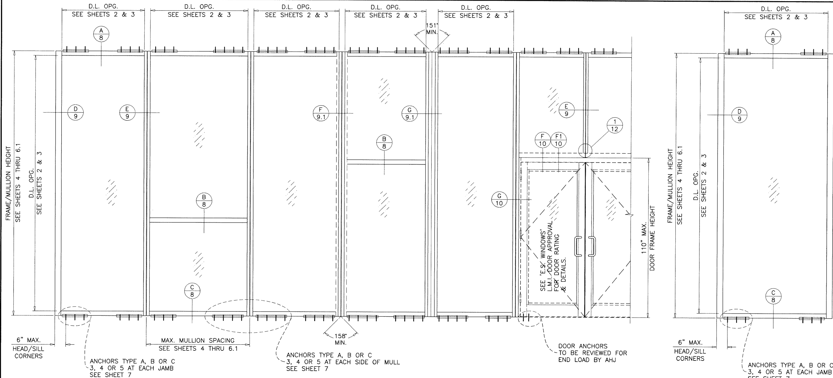
TYPICAL ELEVATIONS
