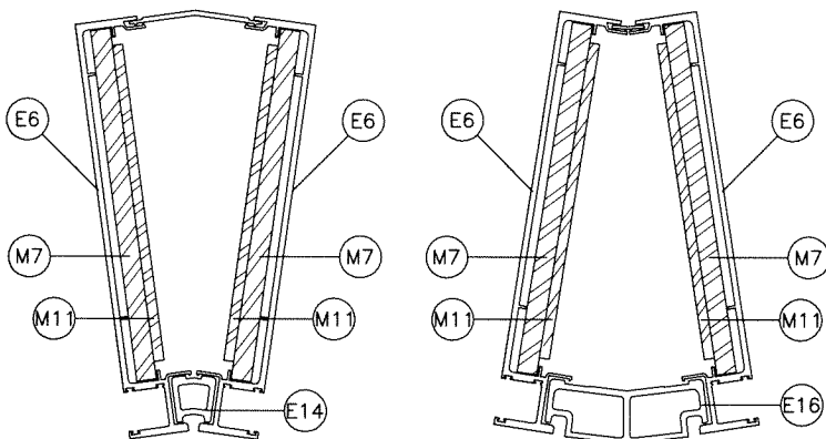
22° BAY MULLION '22 BM2' 30° BAY MULLION '30 BM2'
