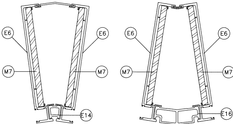
22° BAY MULLION '22 BM1' 30° BAY MULLION '30 BM1'
